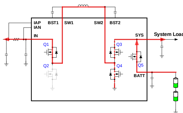
Figure 5: Power FETs' State in OTG Mode
